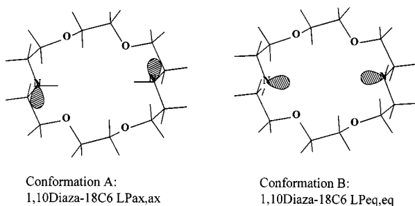
Scheme 2a. Force field calculated conformation of 1,10DA-18C6 2a : A with axial position of lone pairs; B with equatorial positions of lone pairs.
