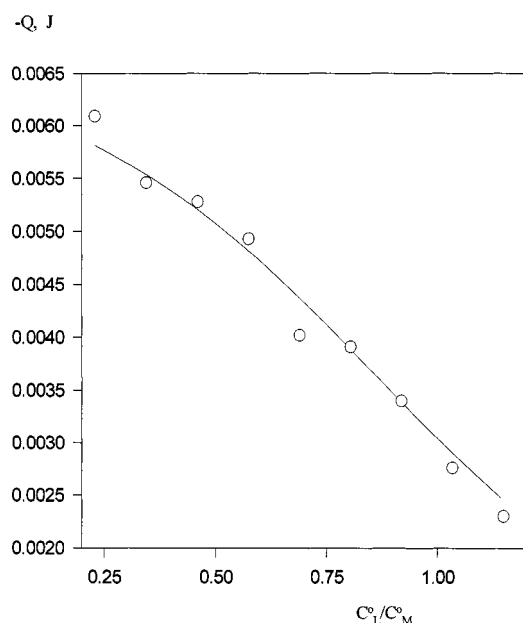
Figure 5a. Calorimetric titration curve for the complexation of 1,10-diaza-18C6 2a with KOH in MeOH at 298 K. Experimental interaction heats (cycles) and calculated titration curve vs. the reagents concentration ratio C_L^0/C_M^0 . Experimental data: the ligand solution ( C_L^0 80.7 mM and \Delta V 0.0212 ml for each point) was added into the mixture ( C_M^0 5.8 mM, C_L^0 0.84 mM, V_0 2.02 ml).
