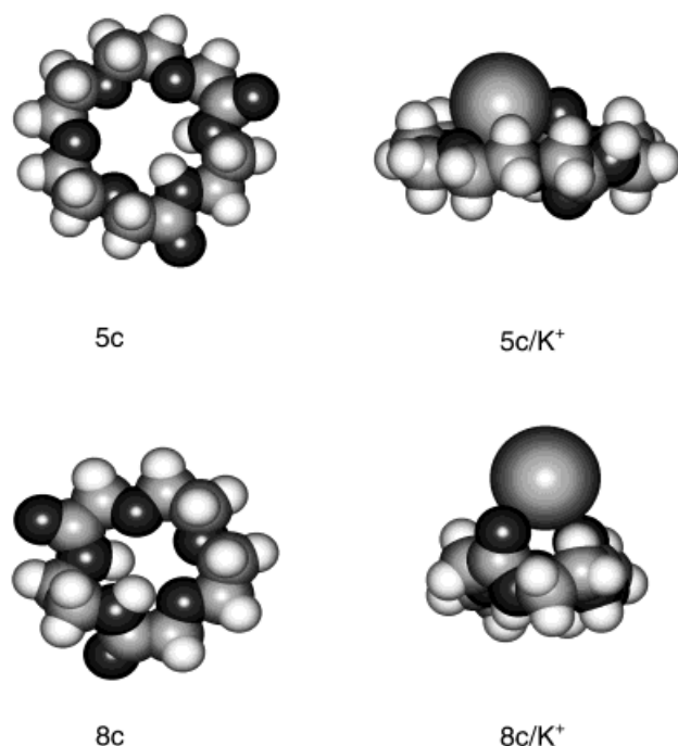
Figure 4. Quanta/CHARMm-minimized structures of amide-crown structures 5c and 8c and their K^+ complexes.
