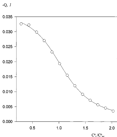
Figure 5b. Calorimetric titration curve for the complexation of 1,7-di(methylaza)-15-crown-5 4b with KCl in MeOH at 298 K. Experimental interaction heats (cycles) and calculated titration curve vs. the reagents concentration ratio C_L^0/C_M^0 . Experimental data: the ligand solution ( C_L^0 277 mM and \Delta V 0.0106 ml for each point) added to the mixture ( C_M^0 12.8 mM, C_L^0 1.5 mM, V_0 2.01 ml).
