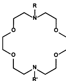
Scheme 1. Structures of ligands, with -\Delta G values —in italics— [kJ/mol] of complexation with K^+ in methanol (other values see Table 1).
