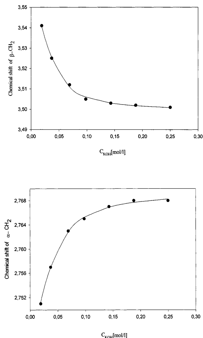
Figure 2. Experimental NMR shifts (dots) and fitted line for the NMR titration of 1,10-diaza 18C6 ( 2a ) with KOH in [D_4]MeOH at 298 K. Association constant: 93 \pm 8 ; \Delta G = -11.2 \text{ kJ mol}^{-1} ; shifts at 100% complexation from fit: CIS ( \alpha ) = 0.024 ppm, CIS ( \beta ) = 0.064 ppm.
