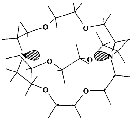
Scheme 2b. LP in,in Conformation of Cryptand [ 222 ]
