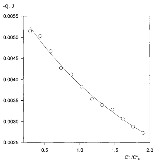
Figure 5c. Calorimetric titration curve for the complexation of 1,10-diaza-21-crown-7 10 with KNO 3 in MeOH at 298 K. Experimental interaction heats (cycles) and calculated titration curve vs. the reagents concentration ratio C_L^0/C_M^0 . Experimental data: ligand solution ( C_L^0 95.1 mM and \Delta V 0.0212 ml for each point) was added to the titrated mixture ( C_M^0 6.8 mM, C_L^0 1.0 mM, V_0 2.02 ml).
