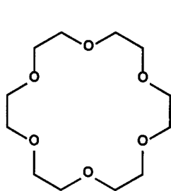
Scheme 1. Structures of ligands, with -\Delta G values —in italics— [kJ/mol] of complexation with K^+ in methanol (other values see Table 1).
