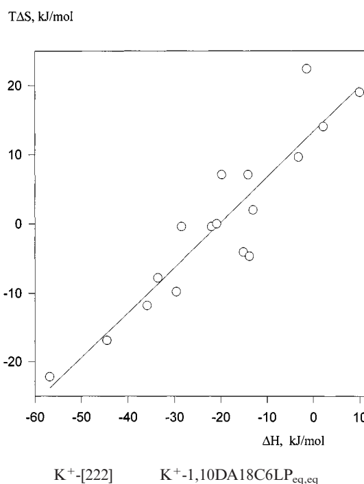
Figure 3. Correlation between \Delta H and T\Delta S for the complexation of K^+ with aza crown ethers, aza oxo crown ethers (amide crowns), 18-crown-6 and 15-crown-5 in MeOH for the K^+ + L \rightleftharpoons (K^+)L equilibrium: T\Delta S = 13.2(3.9) + 0.65(0.15) \Delta H , N = 17 , R = 0.923 , F = 86.5 , SD = 4.8 .
