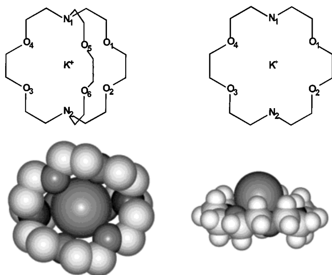
Figure 1. Geometries of the 1,10DA 18C6-LP ax,ax - ( 2a ), 1,10DA 18C6-LP eq,eq - ( 2a ) and cryptand [ 2.2.2 ]-potassium complexes, from CHARMM calculations.
